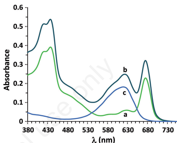
Fig. 2. Absorbance spectra of a) a phosphate buffer extract of “phycobiliprotein-free” pellet suspension of M. aeruginosa (green curve); b) the same amount of pellet suspension extracted diluting it in phycobiliprotein buffer solution (blue-green curve); c) the spectrum of the pure phycobiliproteins is also shown (blue curve). Phycobiliproteins in (b) (blue-green curve) and (c) (blue curve) have the same concentration.
