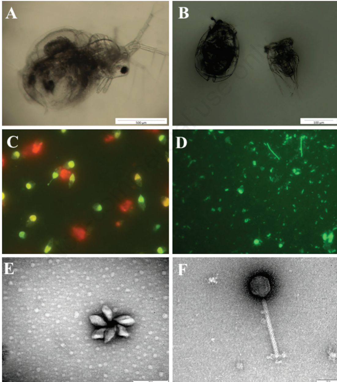
Fig. 4. Images of zoo-, phyto-, bacterio-, and viroplankton diversity in salt lakes of Transylvania: cladocerans ( Moina salina , female) (A) and rotifers from Ursu Lake (Sovata) (B); epifluorescence microscopy of unicellular algae from Brâncoveanu Lake (Ocna Sibiului) (C); various microbial morphotypes in Tarzan Lake (Turda) observed in DAPI-stained samples (D); transmission electron microscopy of spindle-shaped (E) and isometric (F) viruses from Fără Fund lake (Ocna Sibiului). Scale bars: A) 500 µm; B), 100 µm; E) 200 nm; F) 100 nm.
