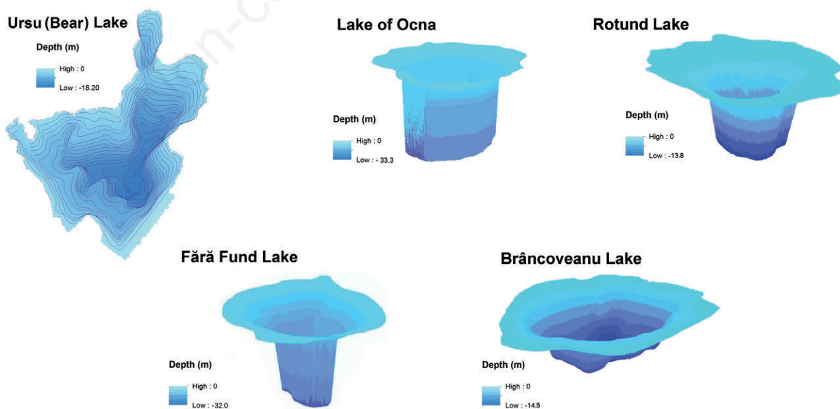
Fig. 2. Three dimensional images of the best investigated lakes to date: Ursu Lake (Sovata area), Ocnei and Rotund lakes (Turda area), Fără Fund and Brâncoveanu lakes (Ocna Sibiului area).
