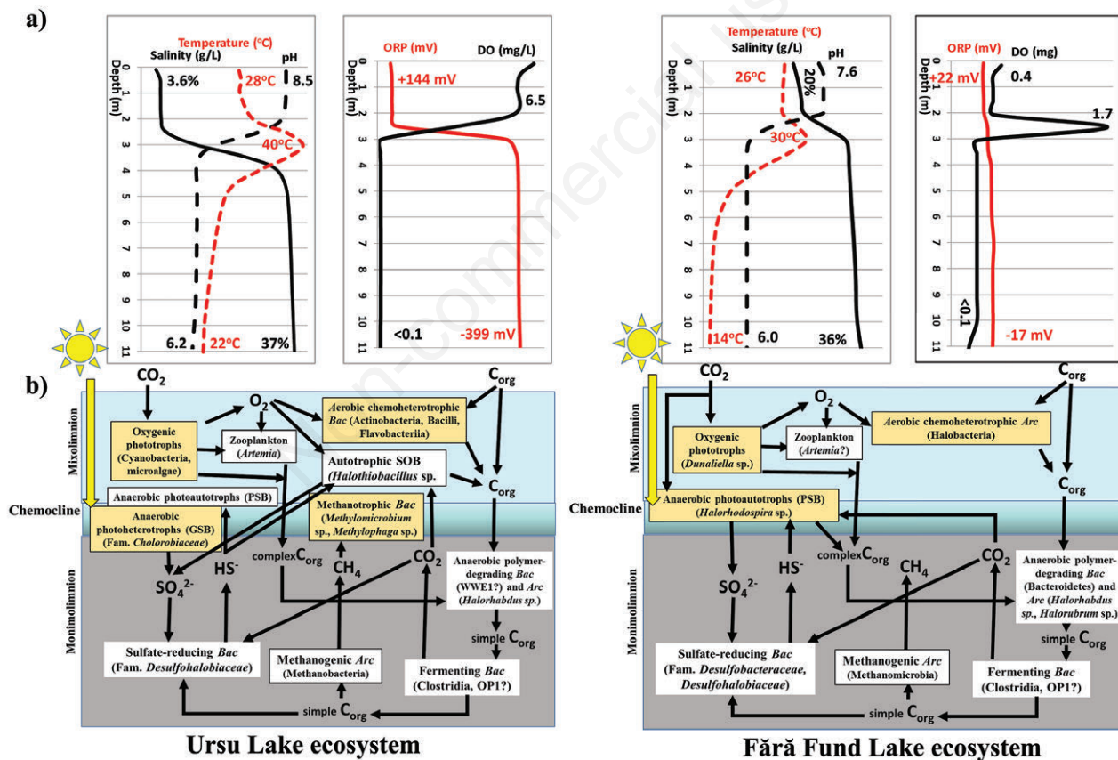
Fig. 3. a) Physico-chemical stratification of Ursu (left) and Fără Fund lakes (right) during 2015 summer season. The heliothermy is observable as temperature peak below surface; relevant values for salinity (black line), temperature (red dotted line), pH (black dotted line), DO (black line), and ORP (red line) are shown. b) The proposed biogeochemical cycling of carbon and sulfur in two aquatic meromictic systems, Ursu (left) and Fără Fund (right), based on DNA metabarcoding approach employed by Andrei et al. (2015). The metabolic groups that differed among two lakes are highlighted in red background. DO, dissolved oxygen concentration; ORP, oxidoreduction potential; C org , organic carbon (complex C org - polymeric substances of plant or animal origin; simple C org , monomers used by fermenters and 1C or 2/3C fermentation products, respectively); Arc, Archaea ; Bac, Bacteria ; SOB, sulfur-oxidizing bacteria.
