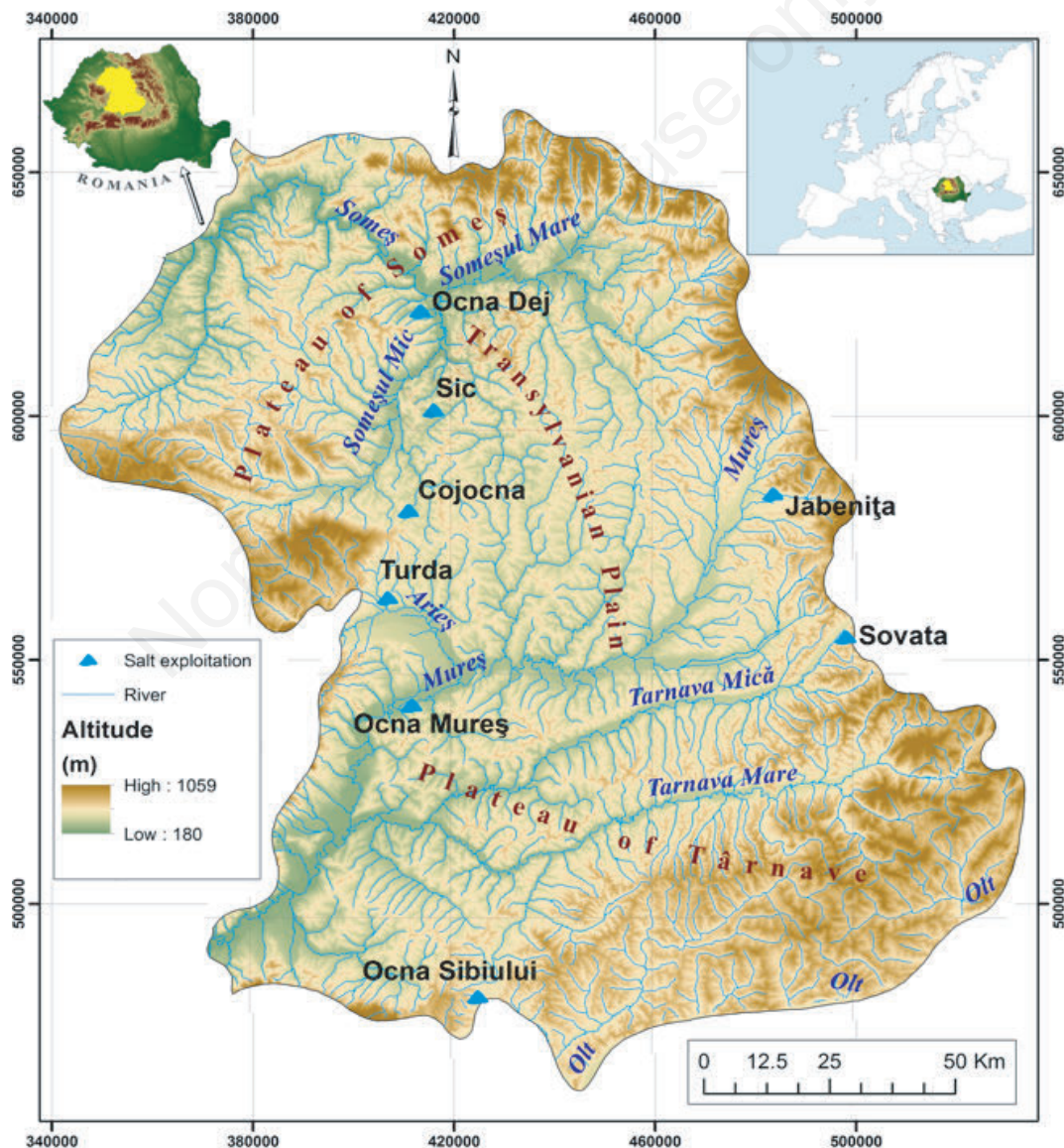
Fig. 1. Locations of salt lakes in the Transylvanian Basin at local (center), Romania (upper left) and Europe scales (upper right).
