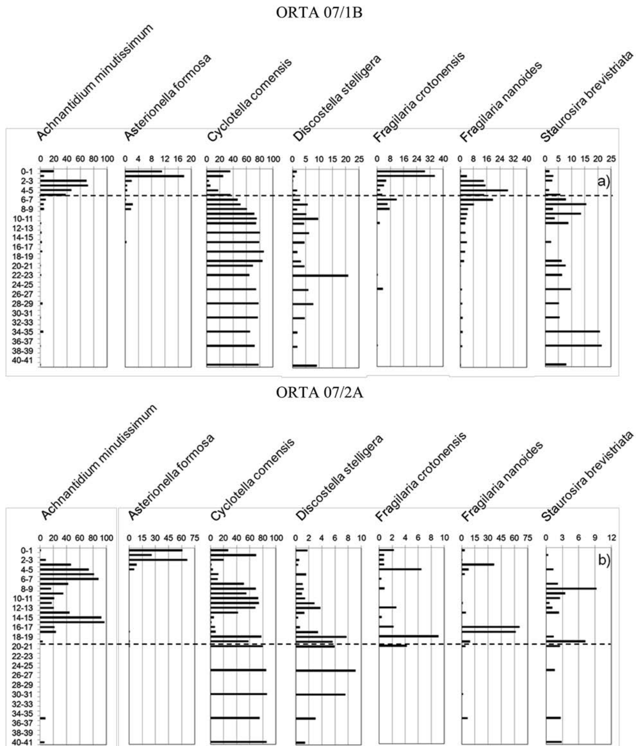
Fig. 3. Profiles of diatom percent abundances along cores ORTA 07/1B (a) and ORTA 07/2A (b). Abrupt decrease in the abundance of Cyclotella comensis and increase of the metal tolerant Achnanthes minutissimum are observed after the onset of Cu pollution in the second half of the 1920s (dashed horizontal lines). Note that, in core ORTA 07/2A, the sedimentary record has been altered at a depth of about 14 cm (see text for details).
