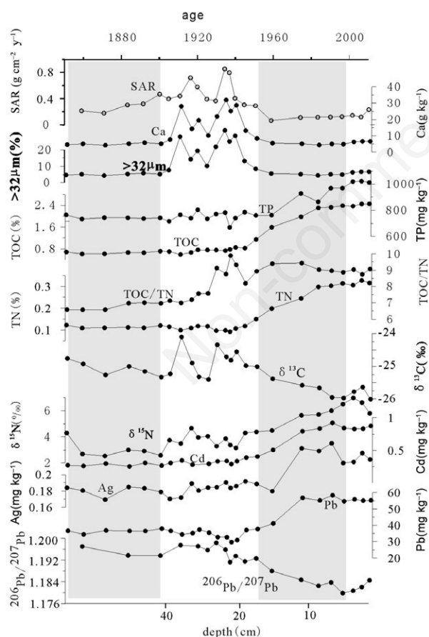
Fig. 3. Summary diagram with time showing sediment accumulation rates (SAR), calcium (Ca), grain size, total organic carbon (TOC), total nitrogen (TN), total phosphorus (TP), TOC/TN, ^{206}\text{Pb}/^{207}\text{Pb} , \delta^{13}\text{C}_{\text{org}} and \delta^{15}\text{N} and heavy metals variations for Huanggaihu Lake.
