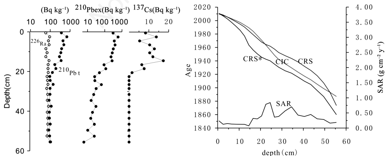
Fig. 2. Vertical profiles of ^{226}\text{Ra} , ^{210}\text{Pbt} (total ^{210}\text{Pb} ), ^{210}\text{Pb}_{\text{ex}} and ^{137}\text{Cs} (left), chronology and sedimentation rate (right) of Huanggaihu Lake. CRS*, composite model derived from the constant rate of supply (CRS) model; CIC, constant initial concentration; SAR, sediment accumulation rates.
