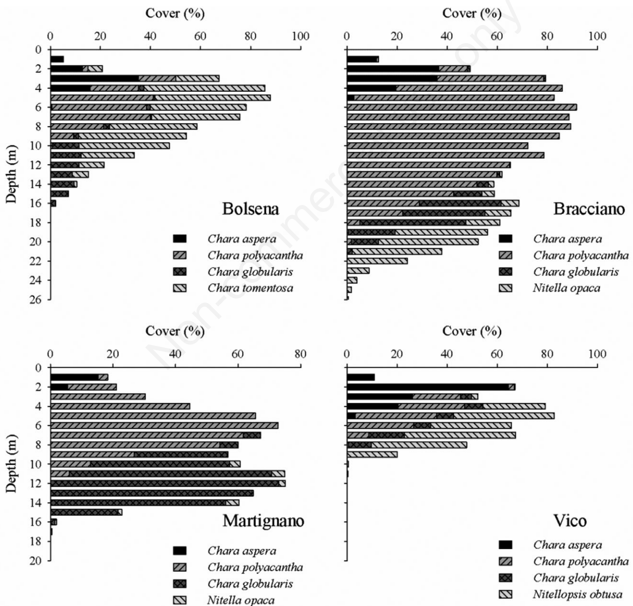
Fig. 3. Distribution of the four most abundant stonewort species in the Chara -dominated Italian volcanic lakes.
