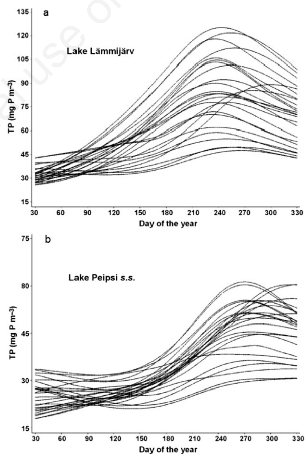
Fig. 5. Seasonal patterns in predicted mean total phosphorus (TP) concentration in Lake Lämmijärv (a) and Lake Peipsi sensu stricto (b) for the 1985-2010 period. Lines correspond to cross-sections of the four-dimensional spline surface fitted to TP by using the year, day within the year, and the two geographical co-ordinates as smoothing factors. Each line shows the surface section for a fixed year; lines in a) are generated by sections through the geographical point 58^{\circ}23'N , 27^{\circ}42'E , while those in b) run through point 58^{\circ}80'N , 27^{\circ}36'E .
