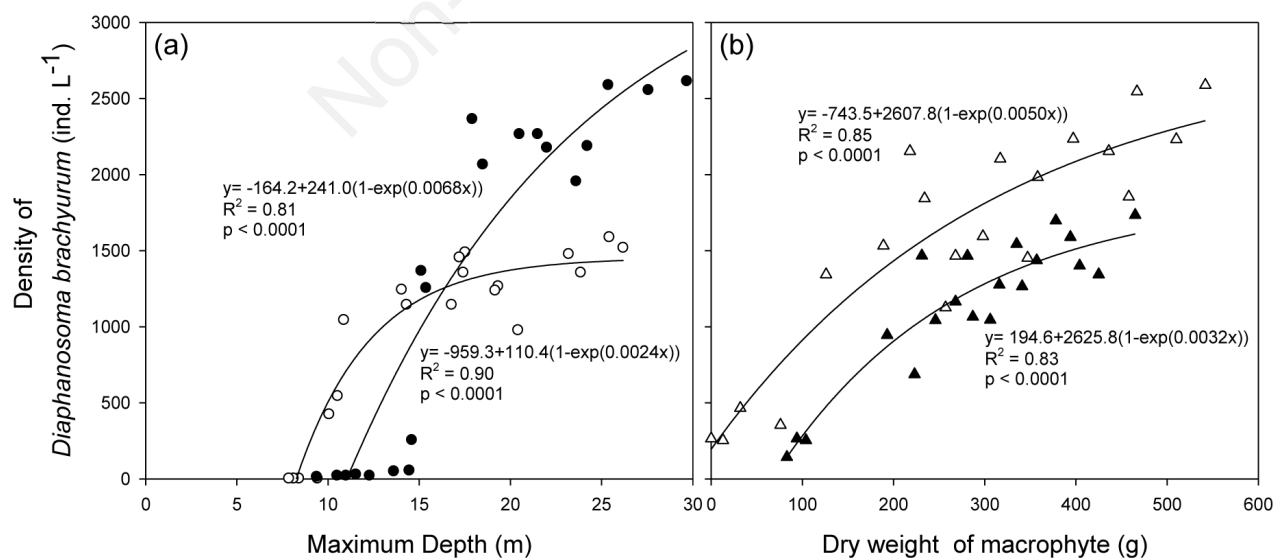
Fig. 4. Regression analysis between Diaphanosoma brachyurum and water body characteristics. White circles in the panel (a) indicate the data from the site 1, and the black circles are for the data of the site 2. White triangles of the panel (b) indicate site 11, and the black triangles were for the site 13.
