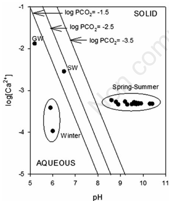
Fig. 6. pH- \log[\text{Ca}^{2+}] diagram showing calcite solution/precipitation equilibrium as \log P_{\text{CO}_2} changes from atmospheric (-3.5) to higher (-2.5 to -1.5) values. As P_{\text{CO}_2} increases there is a drop in pH, and the equilibrium \text{Ca}^{2+}_{\text{max}} line shifts to the left. Winter samples, as well as surface water and ground water remain undersaturated in calcite (see text for details) (based on Deocampo and Ashley, 1999).
