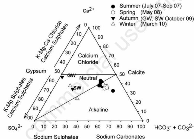
Fig. 5. Plot of the common system \text{Ca}^{2+}\text{-SO}_4^{2-}\text{-(HCO}_3^- + \text{CO}_3^{2-}) in a Spencer triangle. Quantities are expressed in percent milliequivalents \text{L}^{-1} for each vertex component. Note that the October 2009 drought resulted in samples enriched in \text{SO}_4^{2-} and \text{Ca}^{2+} and impoverished in carbonate species relative to the rest.
