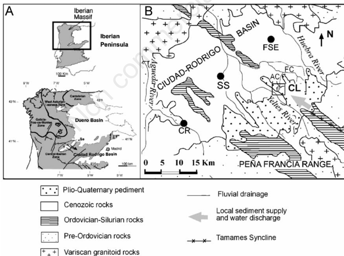
Fig. 1. A) Geological setting of Ciudad Rodrigo basin in the Variscan domains of the Iberian peninsula (after Castro et al. , 2003); B) geological sketch of the Ciudad Rodrigo basin where Cristo lagoon is located. The inset corresponds to Fig. 3. SS, Sancti Spiritus; CR, Ciudad Rodrigo; FSE, Fuente de San Esteban; CL, Cristo lagoon; AC, Aguado creek; FC, Fresneda creek.
