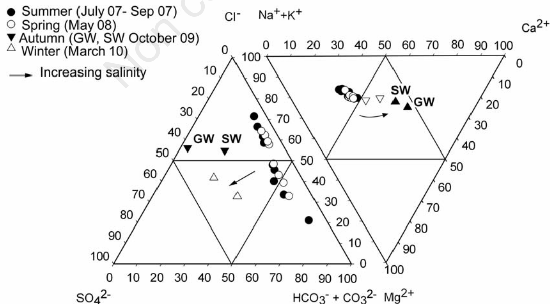
Fig. 4. Composition of the lagoon water in the system \text{Ca}^{2+}\text{-Mg}^{2+}\text{-(Na}^{+}\text{+K}^{+})\text{-(HCO}_3^- + \text{CO}_3^{2-})\text{-Cl}^-\text{-SO}_4^{2-} (percent molar composition for anions and cations).
