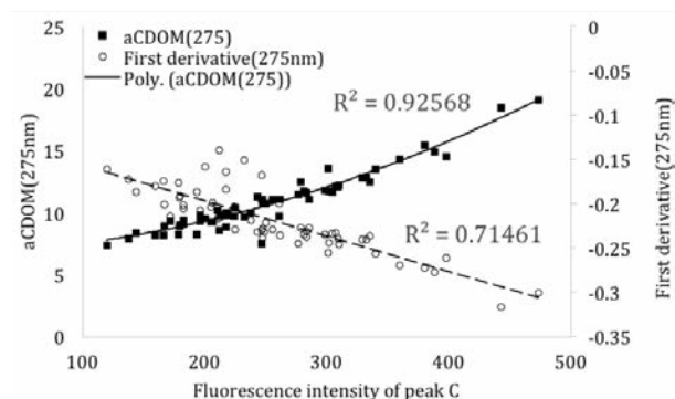
Fig. 5. Relationship between the first derivation value, absorption coefficient and peak C.
