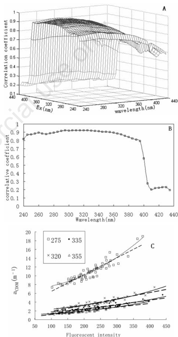
Fig. 6. A, Correlation coefficients between absorption (240~400 nm) and fluorescence intensity (Ex/Em, 240~440 nm/424 nm); B, diagonal representation of A, i.e. the position (wavelength) of absorption and fluorescent is the same; C, relationship between absorption and fluorescence: the unbroken line is the exponential model, while the dashed line represents the linear model.
