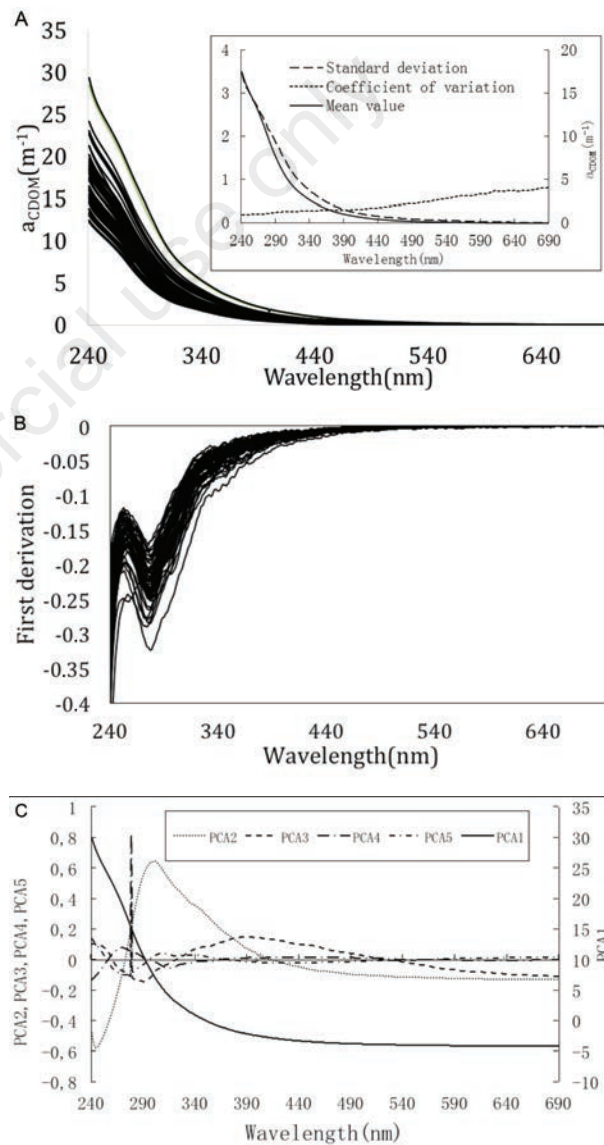
Fig. 2. A, Chromophoric dissolved organic matter absorption spectra ( a_{CDOM} ) in Taihu lake (the figure in top right corner shows the average value, standard deviation and variation coefficient of a_{CDOM} at total sample sites in Taihu lake); B, first derivative of a_{CDOM} ; C, results of the principal component analysis.
