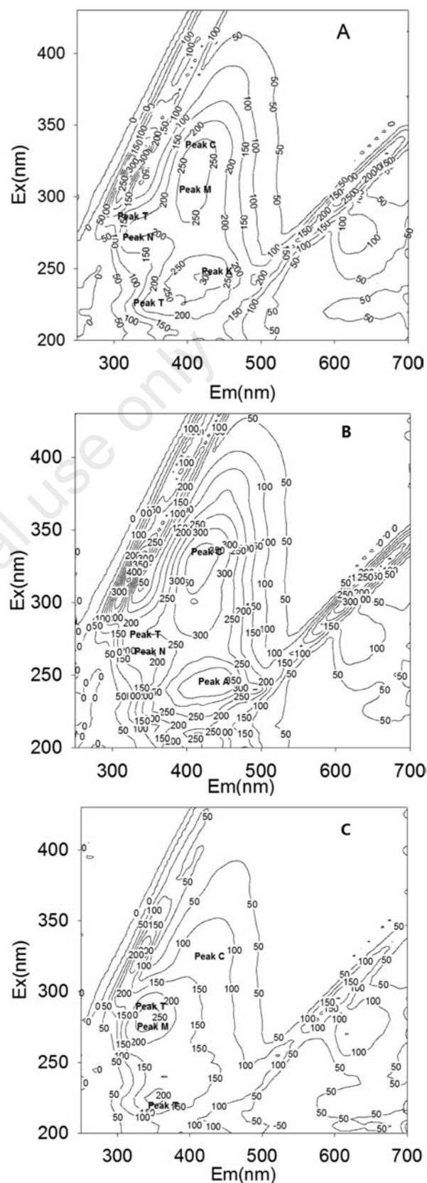
Fig. 3. Total fluorescent peaks identified by three typical styles excitation-emission matrices.
