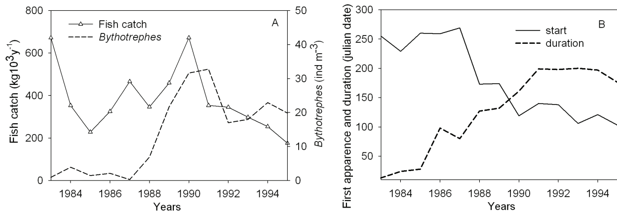
Fig. 2. Changes in mean annual Bythotrephes population density and commercial catch of non-piscivorous fish (data from Grimaldi 1997) (A); time at growing start and of duration of Bythotrephes planktonic population (B).
