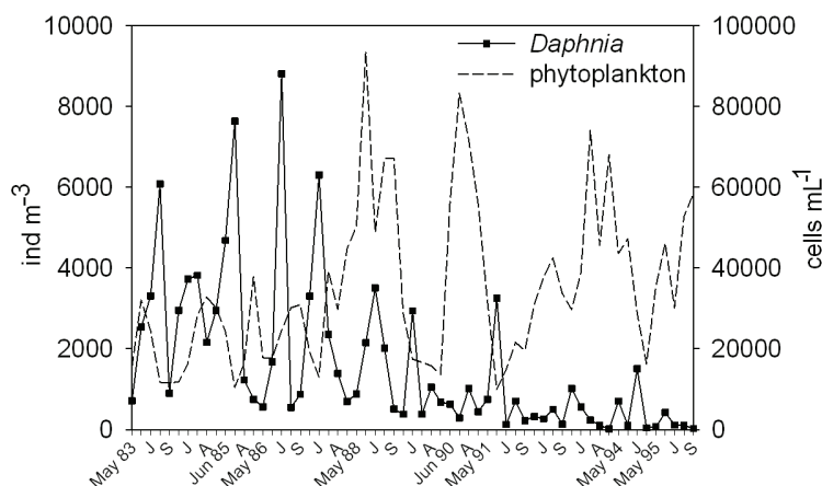
Fig. 4. Changes in Daphnia abundance (May–September) with phytoplankton cell numbers over the period 1983–1995 (from Manca & Ruggiu 1998).
