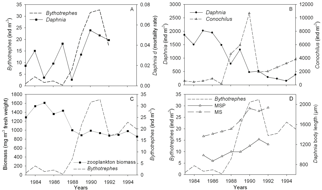
Fig. 3. (A) Bythotrephes population density and Daphnia per capita mortality rate; (B) Daphnia and Conochilus population densities (1983–1995) (from Manca & Sonvico 1996); (C) Bythotrephes abundance and zooplankton biomass; (D) Daphnia body size (length; for explanation of MSP and MS see methods) and Bythotrephes abundance. All panels refer to the period 1983–1995.
