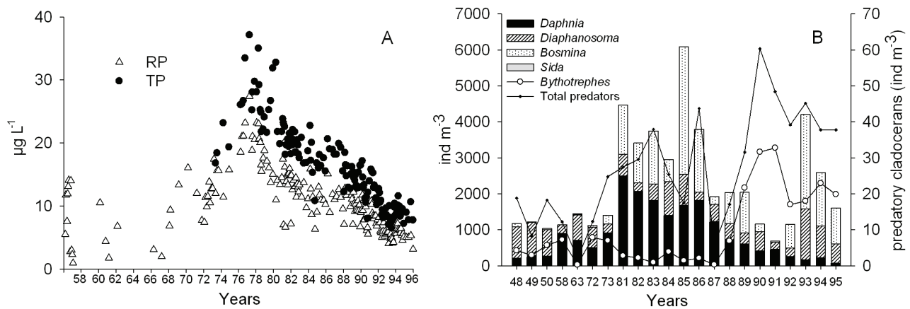
Fig. 1. (A) Long-term changes in total (TP) and reactive (RP) phosphorus concentrations and (B) long-term changes in Cladocera abundance and taxa composition, in Lago Maggiore.
