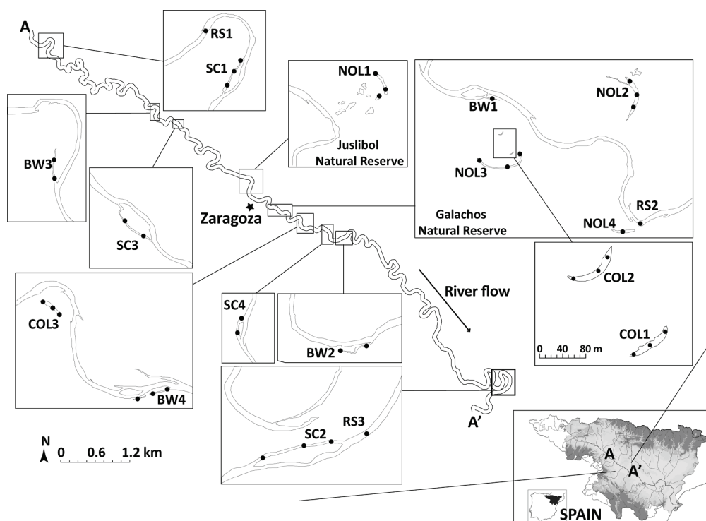
Fig. 1. Study area and site locations. RS = River sites, SC = secondary channels, BW = backwaters, NOL = natural oxbow lakes, COL = constructed oxbow lakes. Scale bar applies to every enlarged area except COL1 and COL2, which are presented on a different scale. Distance from A to A' is approximately 100 km.
