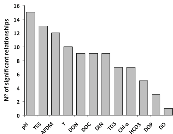
Fig. 3. Number of significant relationships found between each environmental factor and biological trait-categories, obtained by means of the fourth-corner method.
