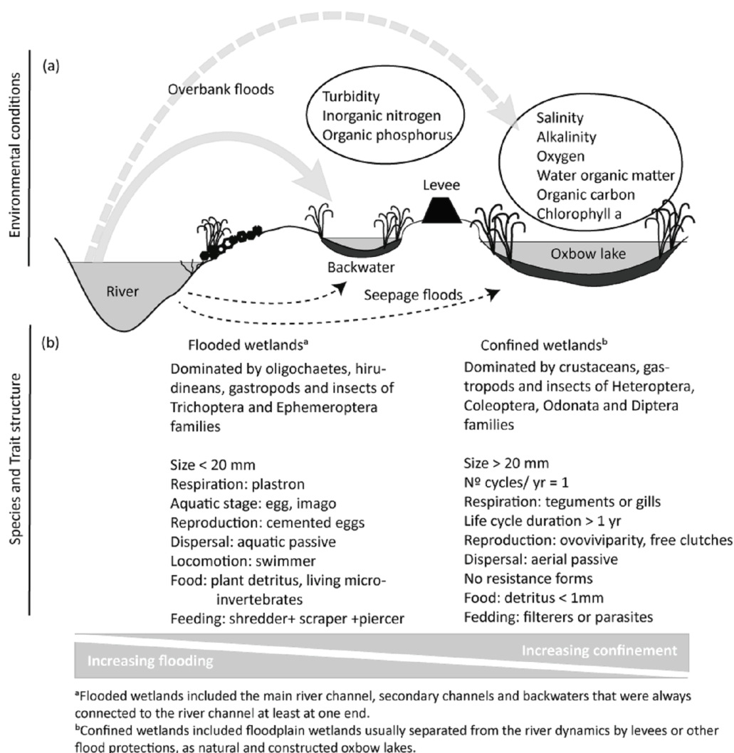
Fig. 5. Template of habitat conditions and response of species and trait structure in the Ebro river-floodplain, based on results from this study. (a) Habitat conditions related to the frequency and duration of flood pulses. (b) Response of the macroinvertebrate species and trait structure to flooding- and confinement-related variables.
