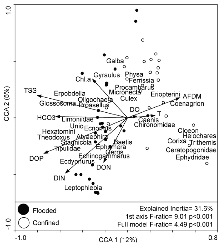
Fig. 2. Results of Canonical Correspondence Analysis performed between species abundance and environmental features in the Ebro river-floodplain.
