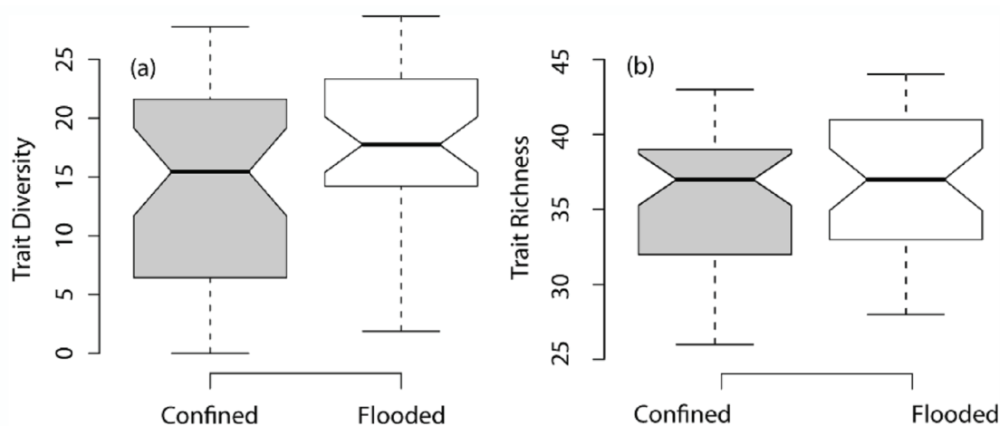
Fig. 4. Trait diversity (a) and richness (b) in flooded and confined sites of the Ebro river-floodplain.
