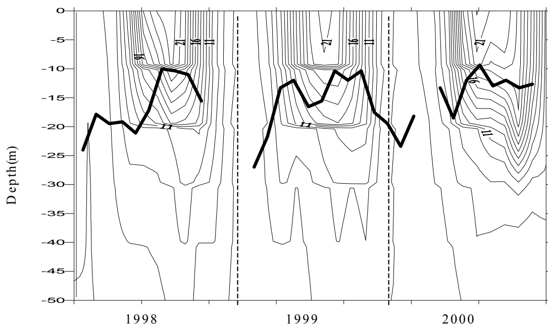
Fig. 2. Isoleths of temperatures ( ^{\circ}\text{C} ) with superimposed seasonal variations of the euphotic depth (m).
