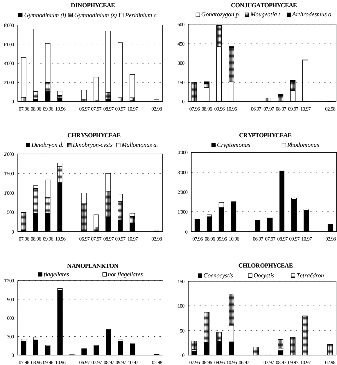
Fig. 2. Biomass of the main phytoplankton taxa [ \text{mg m}^{-2} ; fresh weight].
