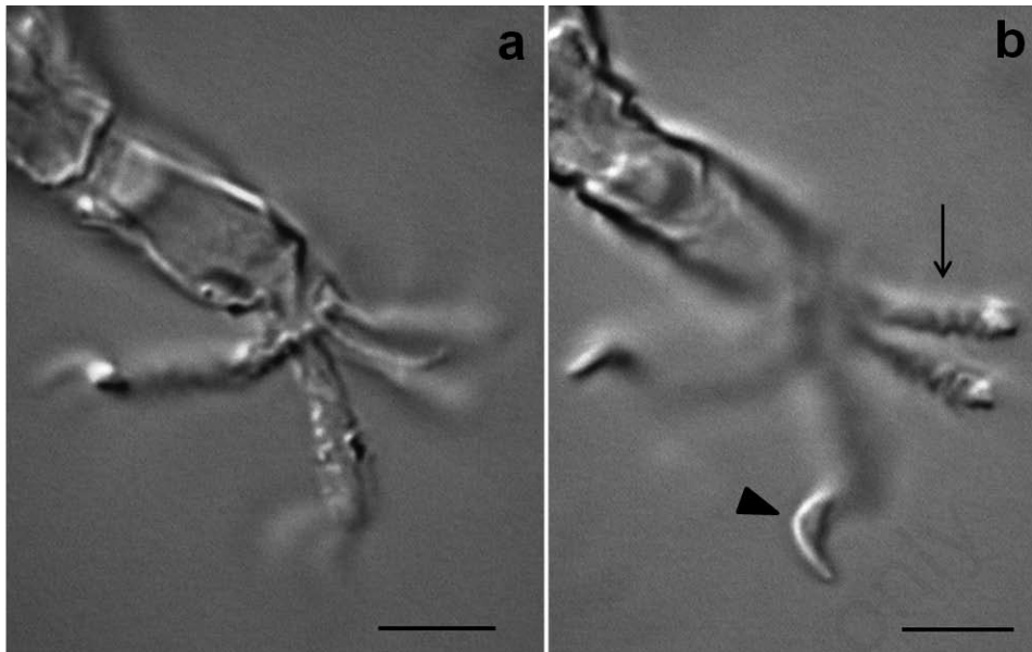
Fig. 3. Prostygarcus aculeatus gen. nov., sp. nov., close up of leg IV of a paratype at different focus positions. a) Detail of the tarsus showing the insertion of digits; b) detail of digits showing wrinkles (arrow) and simple claws (arrowhead). Scale bars=5 \mu m.
