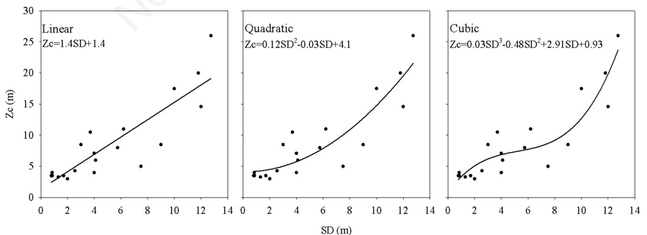
Fig. 2. Linear models used to explain the correlation between Z_c (maximum depth of macrophyte colonization) and SD (Secchi disk transparency). The linear model is on the left, the second-order polynomial (quadratic) in the center, and the third-order polynomial (cubic) model on the right.
